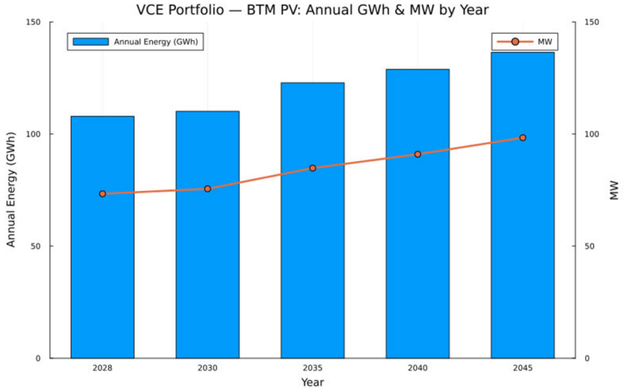
Figure 3 - BTM Solar Forecast: Annual Generation (GWh) and Installed Capacity (MW)
