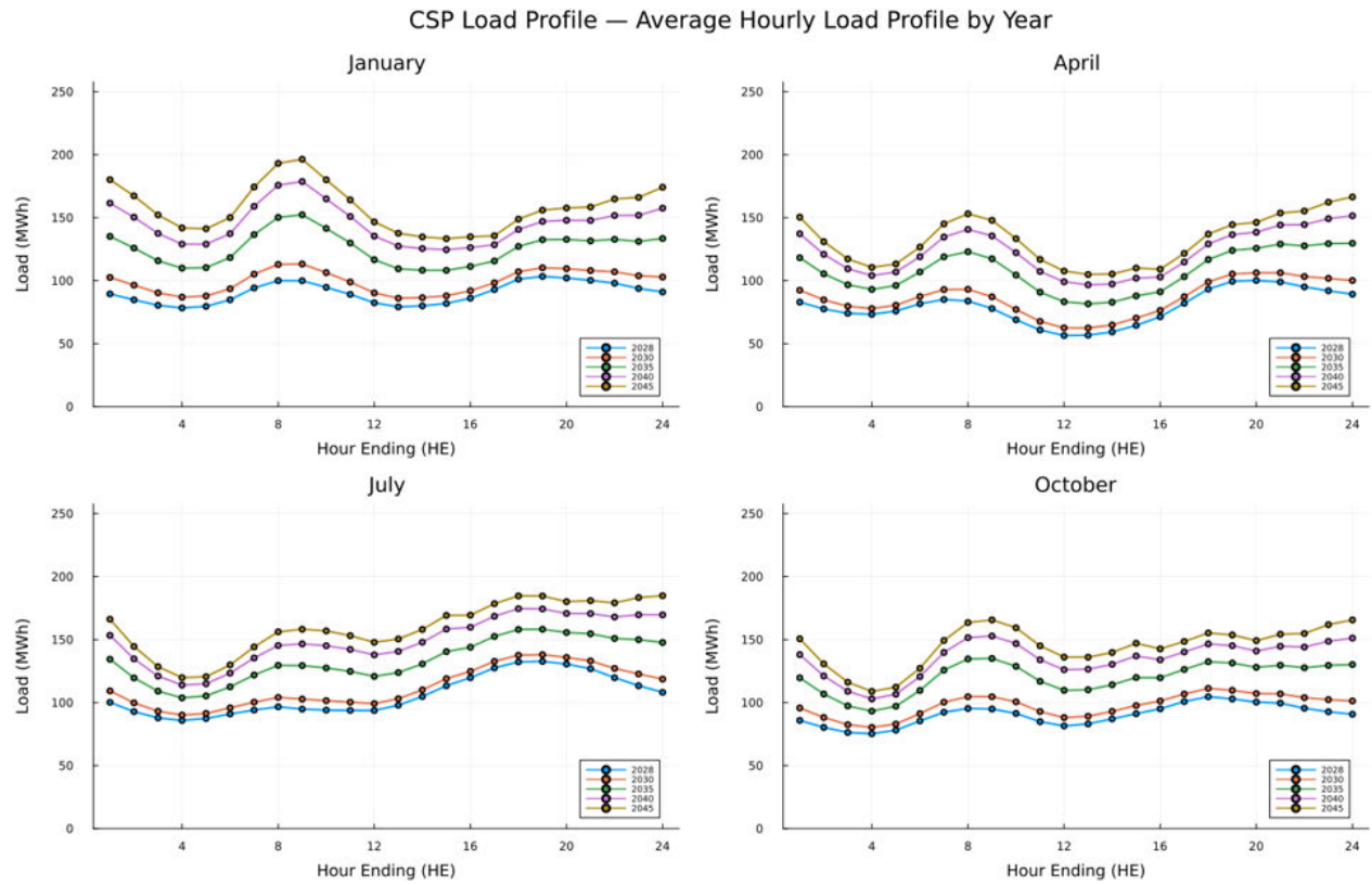
Figure 5 - Monthly Average Hourly Load Profile by CSP Planning Year (CPUC-CSP)
